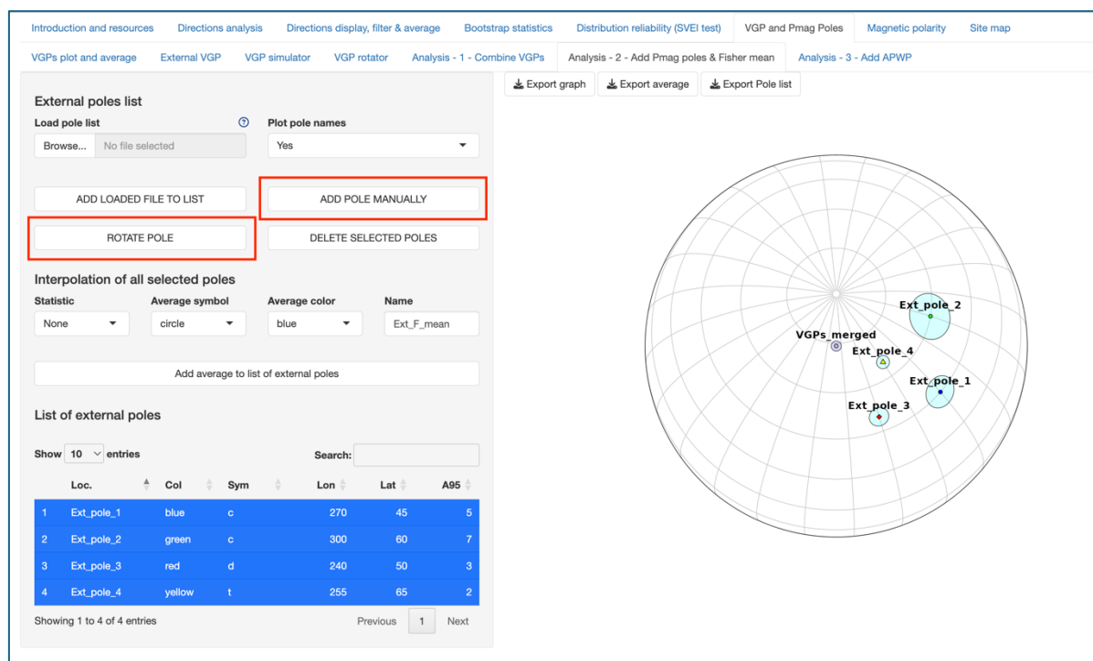
Figure 5.6.1. Analysis – 2 – Add paleomagnetic poles and Fisher mean sub-page. Highlighted the action buttons the open the data entry pop-up window (Figures 5.6.2 and 5.6.3)
