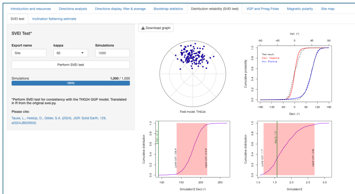
Figure 4.1. SVEI test for consistency with the THG24 GGP model.
