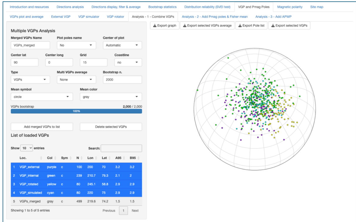
Figure 6.5. Example of merged VGPs.
