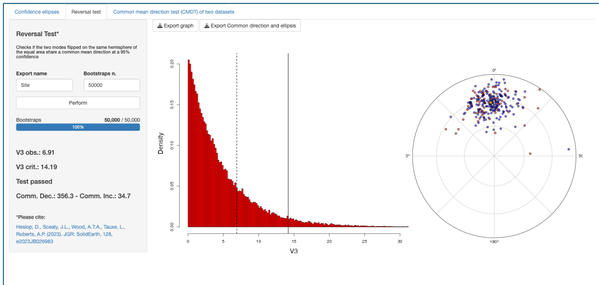
Figure 4.2. Sub-page performing the bootstrap test for a common mean direction applied on the two modes of the same distribution (aka reversal test).
