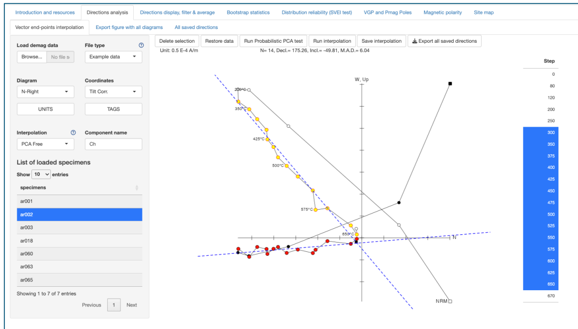
Figure 2.1. Vector end-points interpolation main window.
