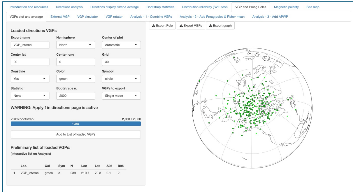
Figure 6.1. VGPs plot and average sub-page.
