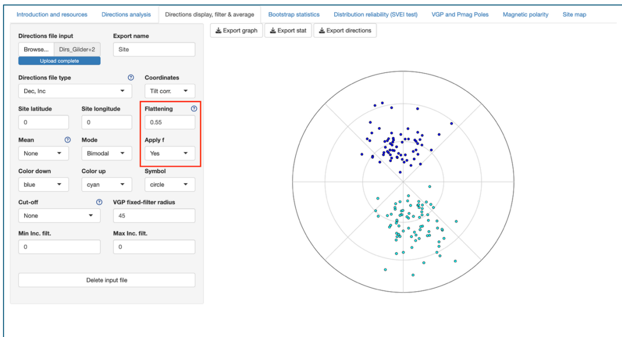
Figure 5.4. The f value is applied to the original dataset.
