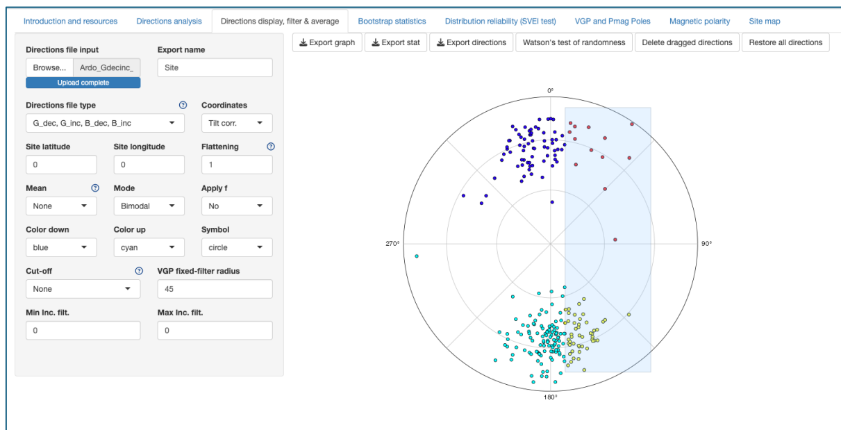
Figure 3.1. Directions display, filter and average window.
