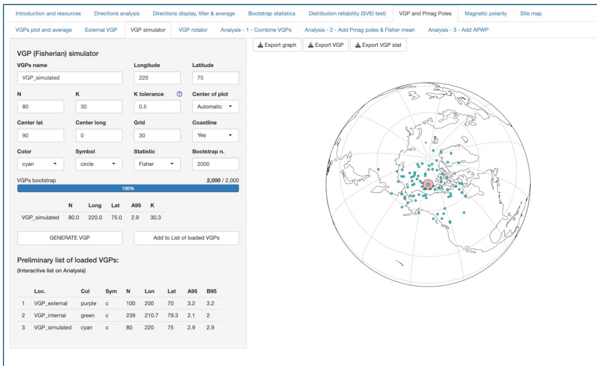
Figure 6.3. Simulated VGPs sub-page.
