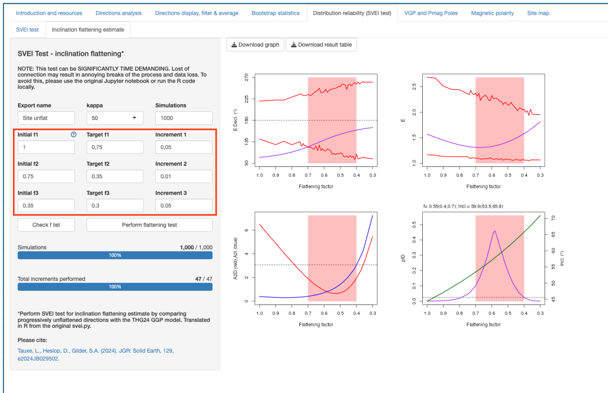
Figure 5.3. Detailed inclination flattening calculation process.
