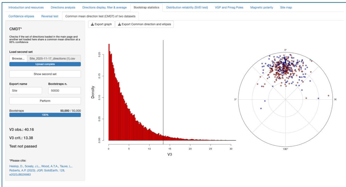
Figure 4.3. Bootstrap-based common mean direction test (CMDT) sub-page.
