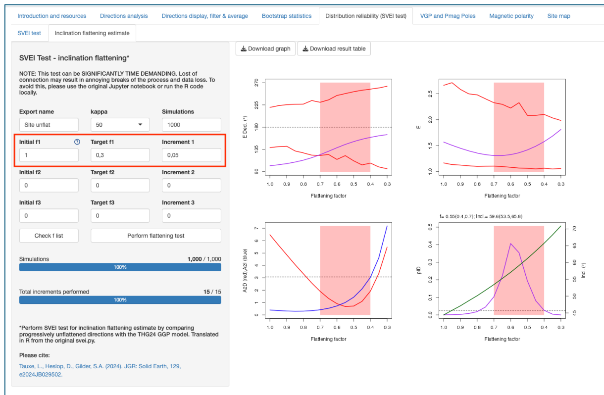
Figure 5.2. Preliminary (explorative) paleomagnetic inclination flattening detection.
