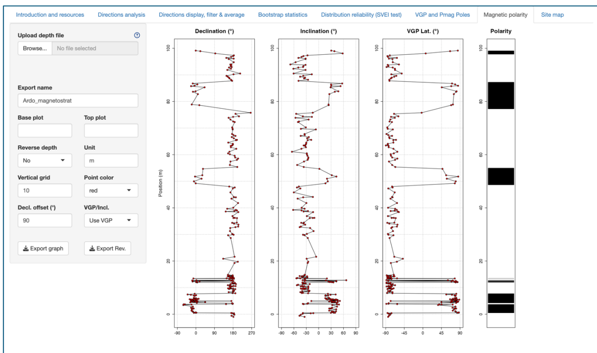
Figure 7.1. Magnetic polarity stratigraphy page
