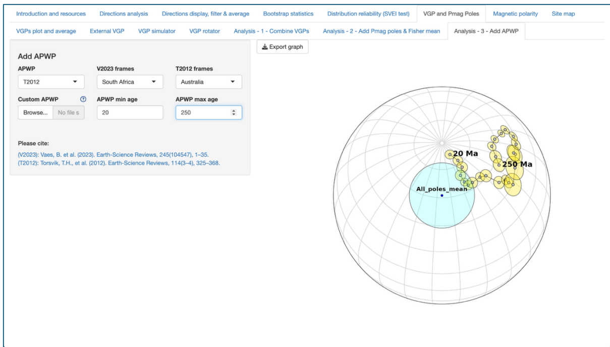
Figure 6.9. Add APWP sub-page.
