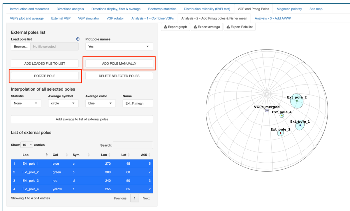
Figure 6.6. Analysis – 2 – Add paleomagnetic poles and Fisher mean sub-page. Highlighted the action buttons the open the data entry pop-up window (Figures 6.7 and 6.8)
