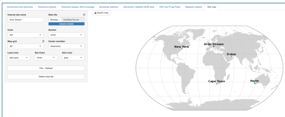
Figure 8.1. Site map page.
