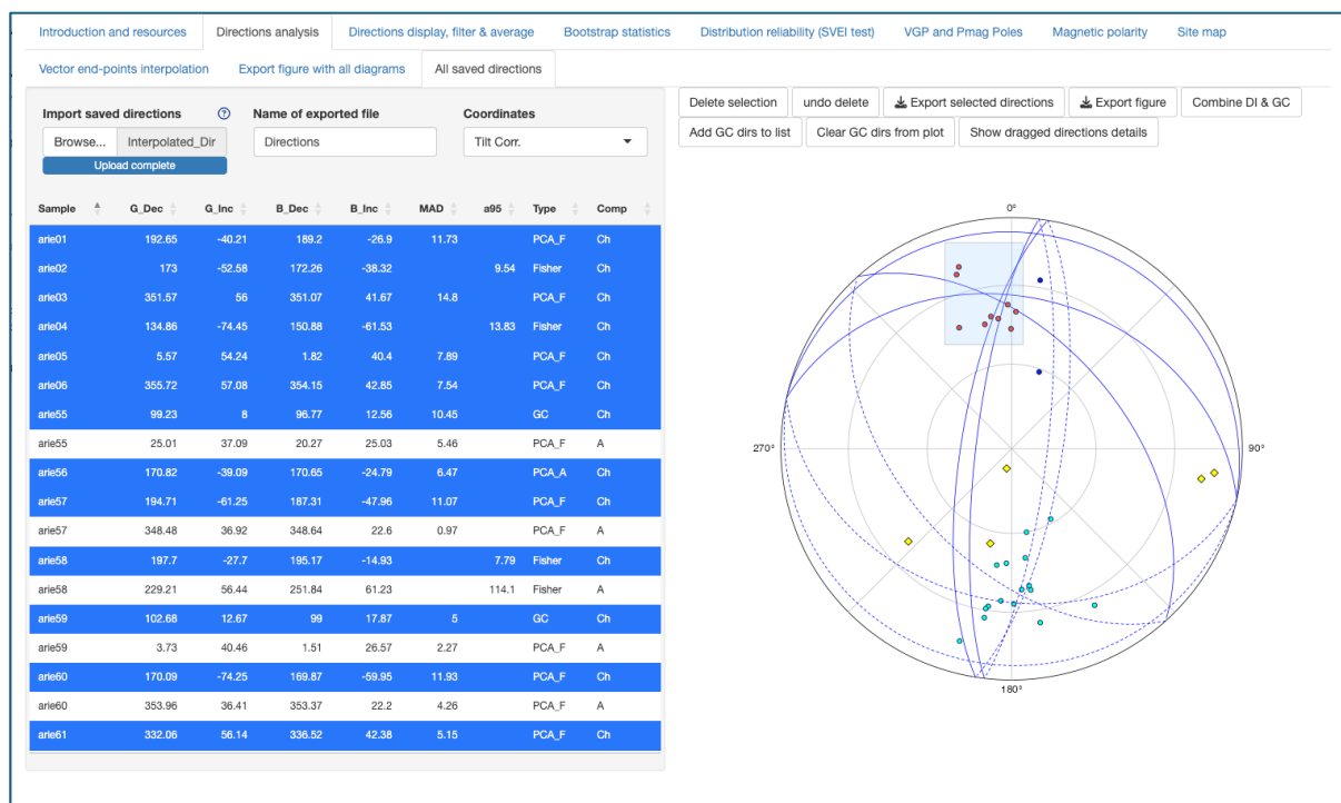
Figure 2.3. Window showing all saved interpolated directions and planes.
