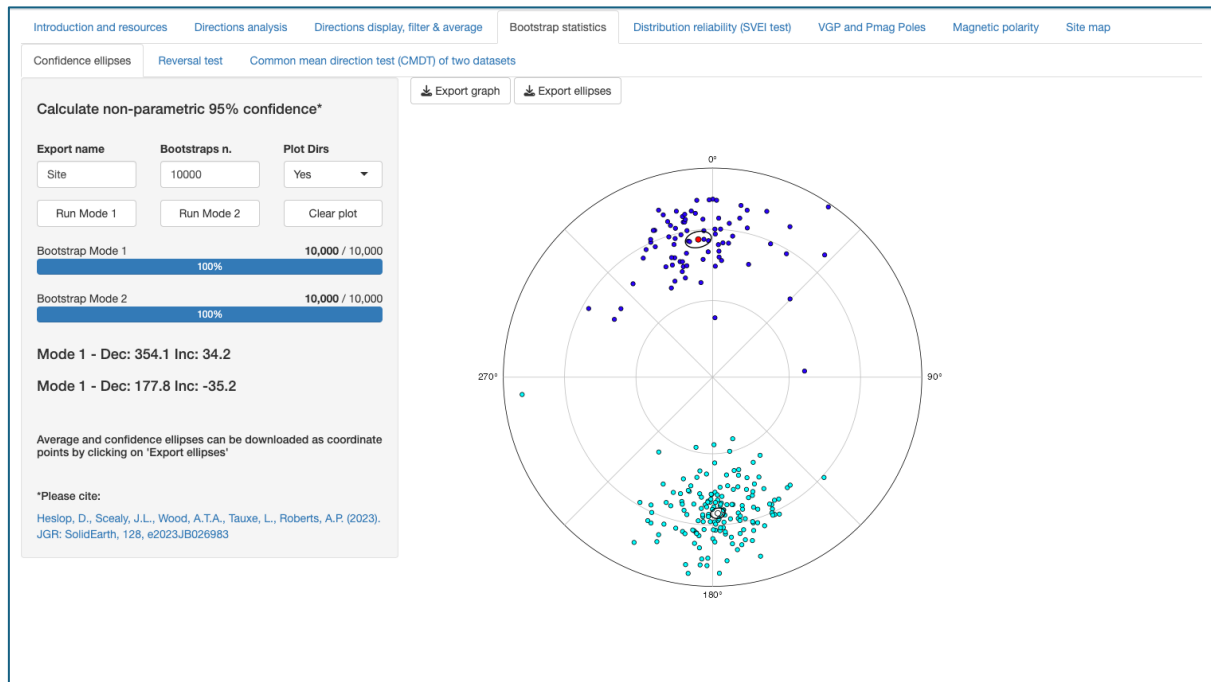
Figure 4.1. Confidence ellipses sub-page of the bootstrap statistics.
