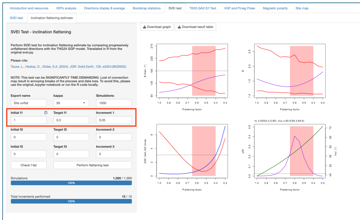
Figure 5.2. Preliminary (explorative) paleomagnetic inclination flattening detection.
