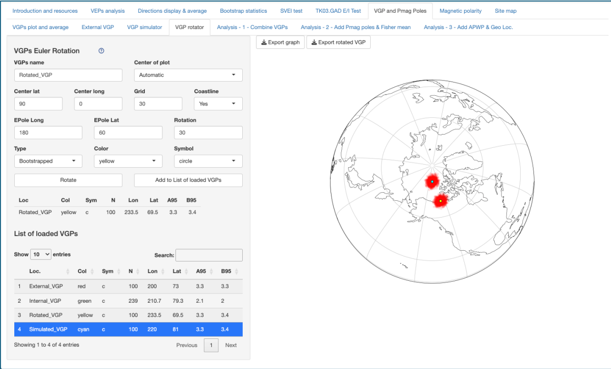
Figure 7.4. VGPs rotation sub-page.
