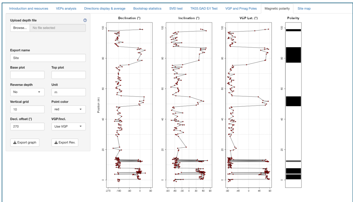
Figure 8.1. Magnetic polarity stratigraphy page
