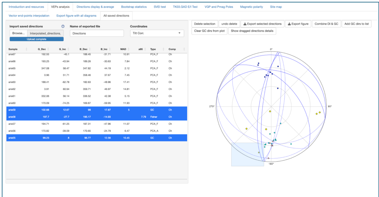
Figure 2.3. Window showing all saved interpolated directions and planes.
