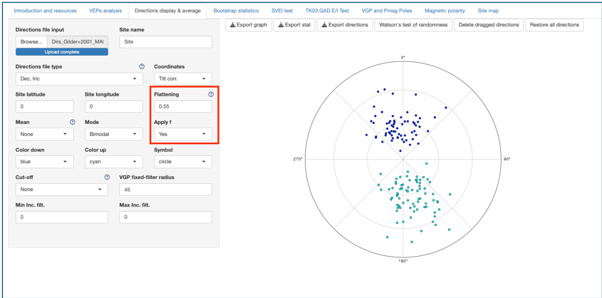
Figure 5.4. The f value is applied to the original dataset.
