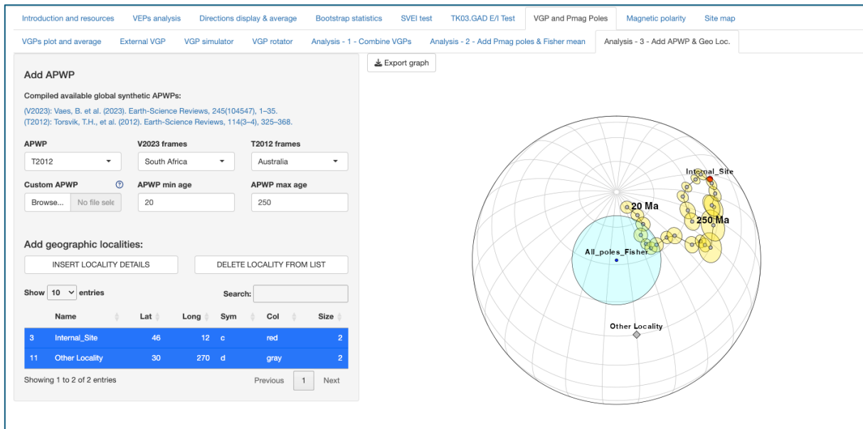
Figure 7.7. Add APWP sub-page.
