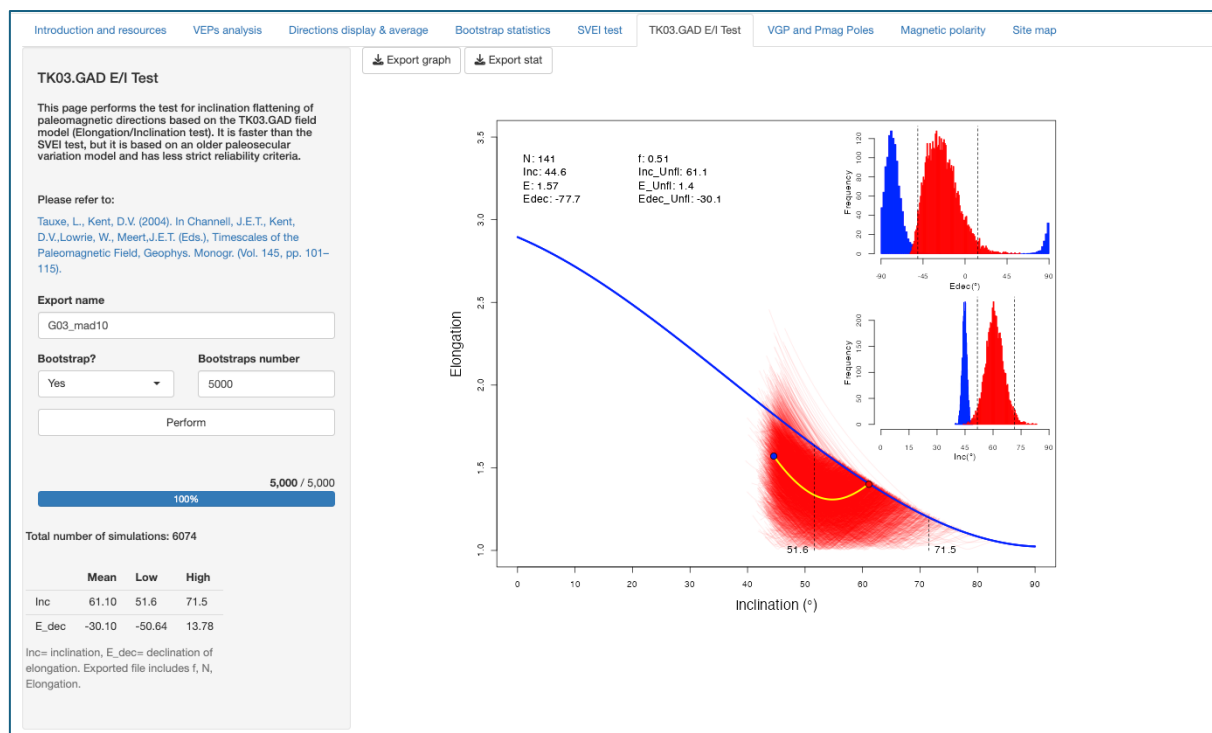
Figure 6.1. TK03.GAD-based inclination shallowing detection and correction.
