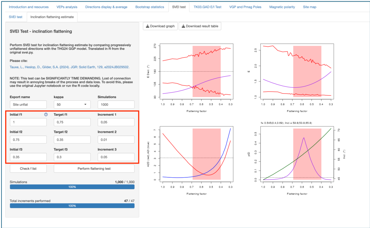
Figure 5.3. Detailed inclination flattening calculation process.
