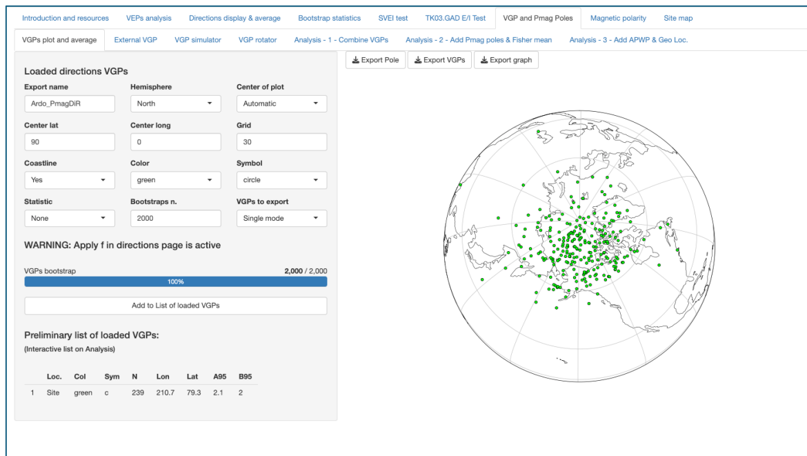
Figure 7.1. VGPs plot and average sub-page.
