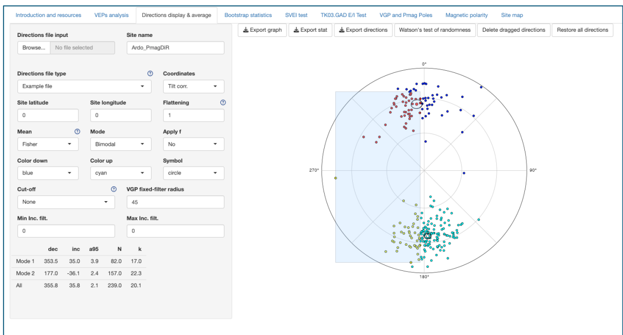
Figure 3.1. Directions display & average window.
