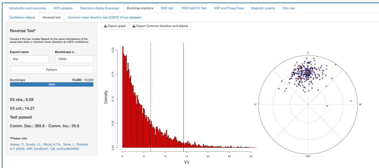
Figure 4.2. Bootstrap test for a common mean direction (aka reversal test) sub-page.
