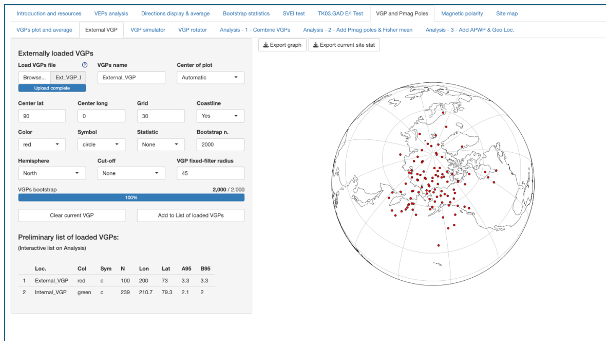
Figure 7.2. External VGPs sub-page.
