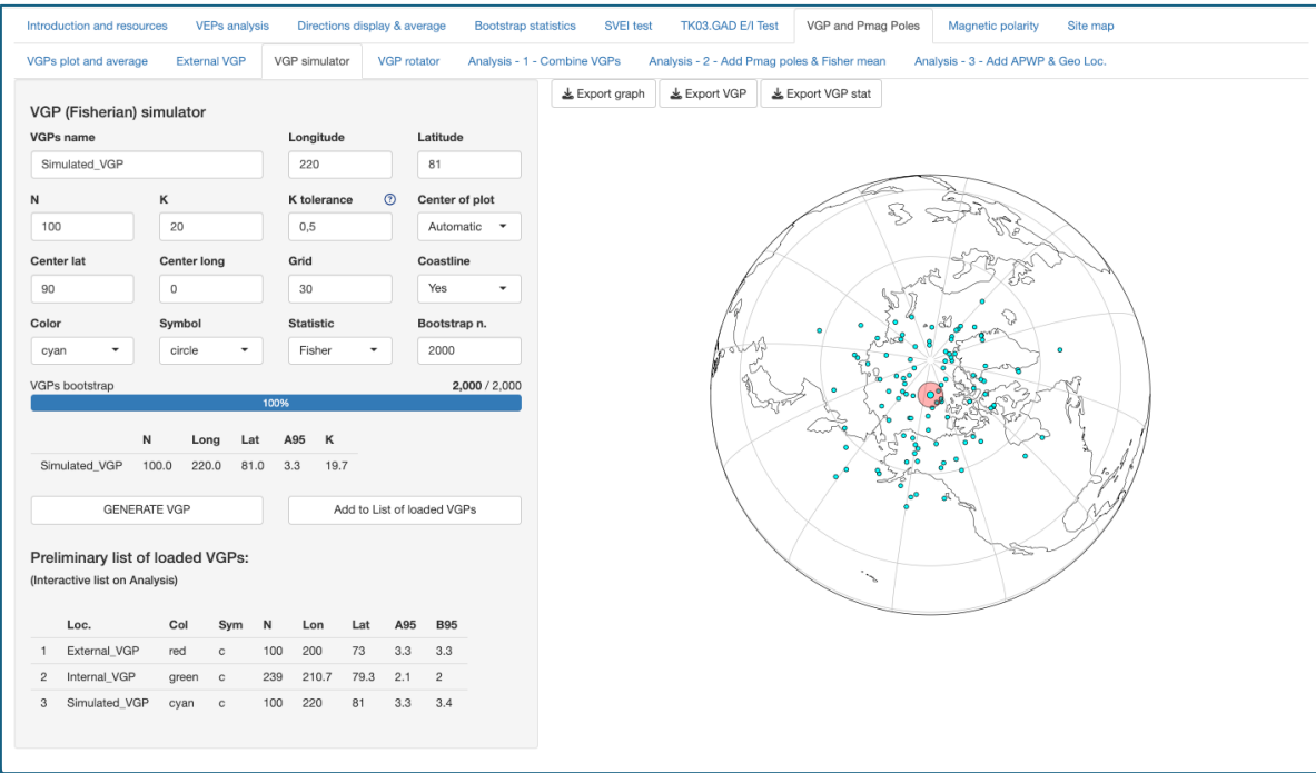
Figure 7.3. Simulated VGPs sub-page.
