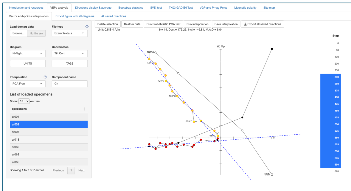
Figure 2.1. Vector end-points interpolation main window.
