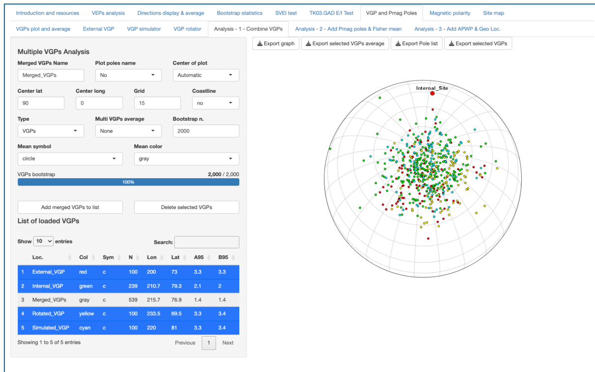
Figure 7.5. Example of merged VGPs.
