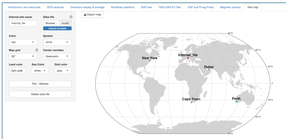
Figure 9.1. Site map page.
