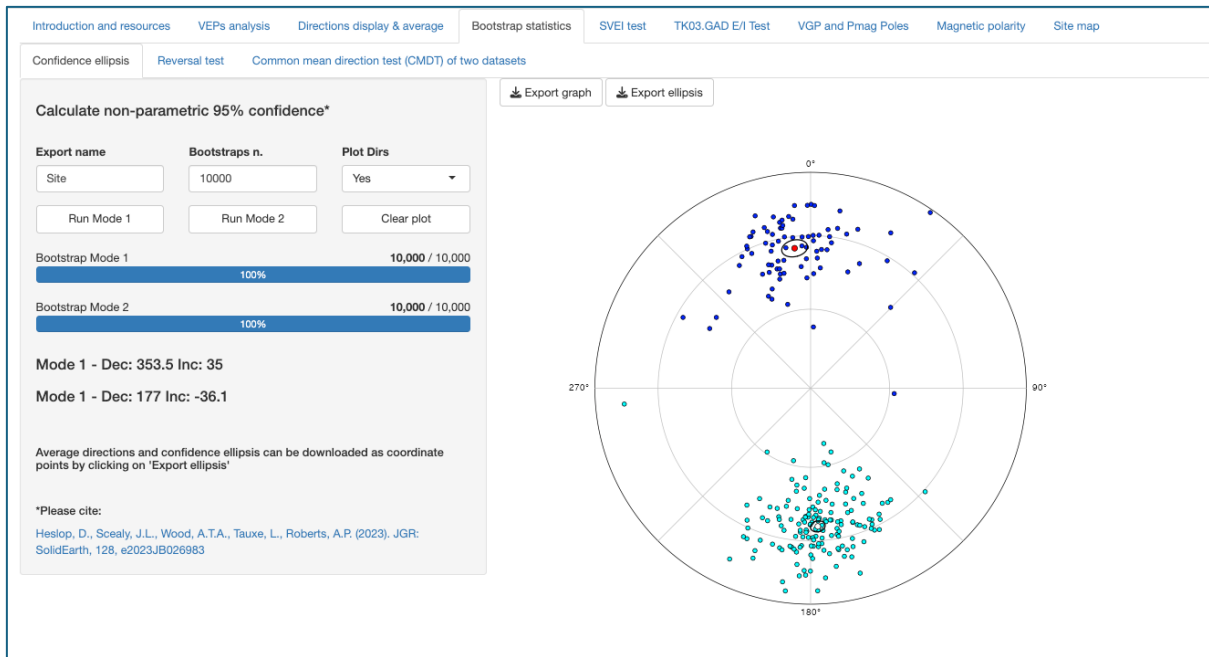
Figure 4.1. Confidence ellipses sub-page of the bootstrap statistics.
