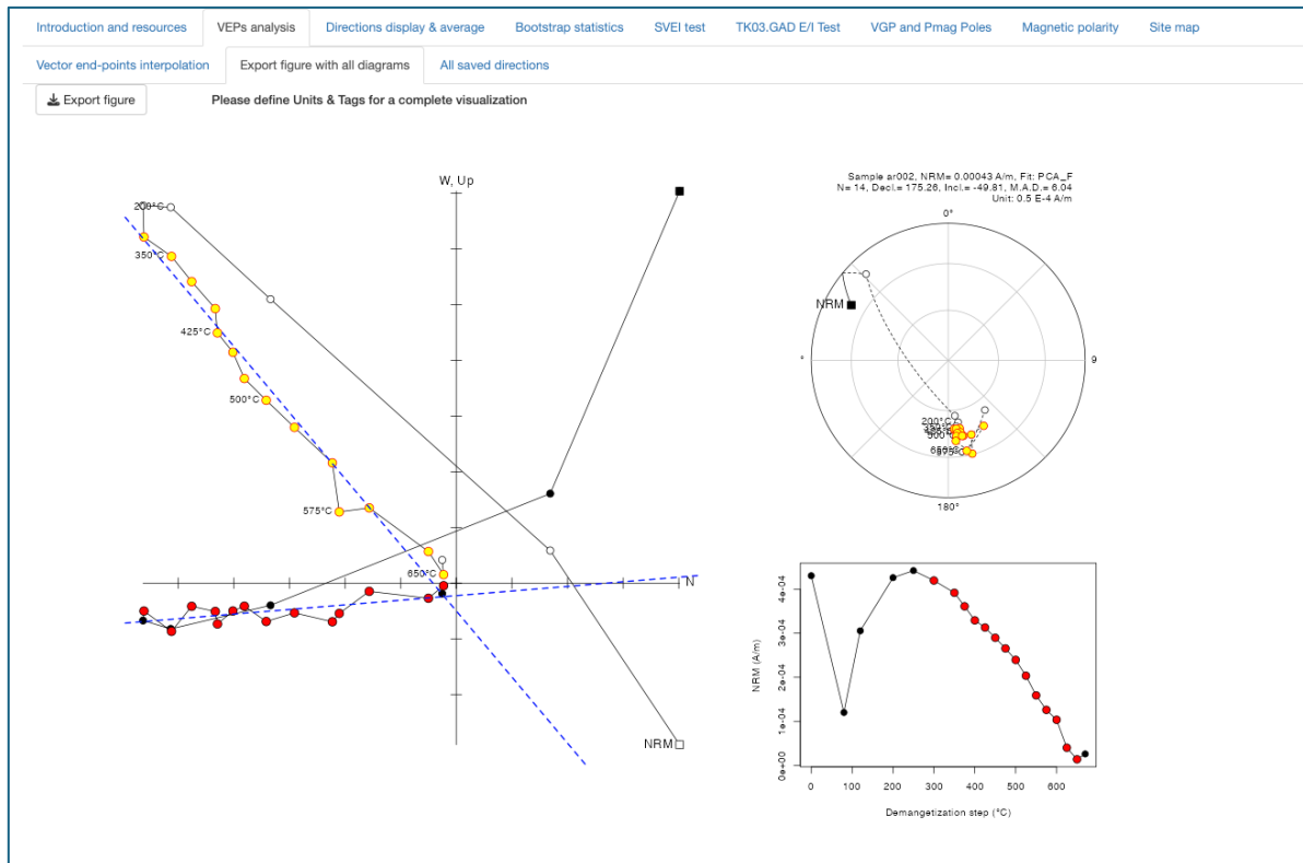
Figure 2.2: window showing all details of the sample selected in the “Vector end-points interpolation” panel, with the details of the interpolated direction (if present).
